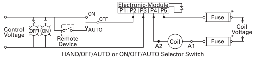
View C Optional Pilot Devices for 3-Wire Control
