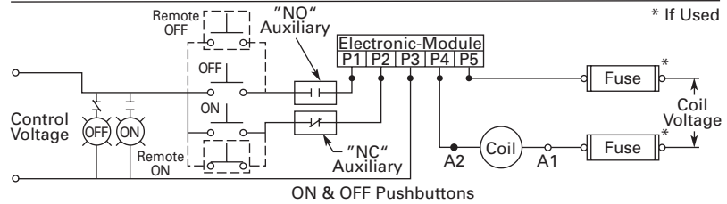
View C Optional Pilot Devices for 3-Wire Control
